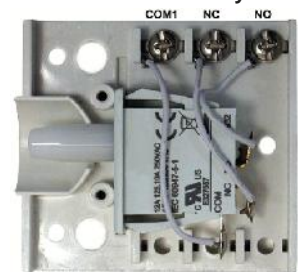
SPDT Momentary
