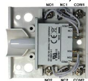
DPDT Momentary
